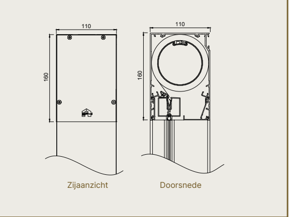
Medium - MS 7B - Kast
