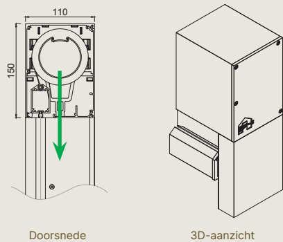
Fixscreen® 100 Slim - MS 7B - Kast
