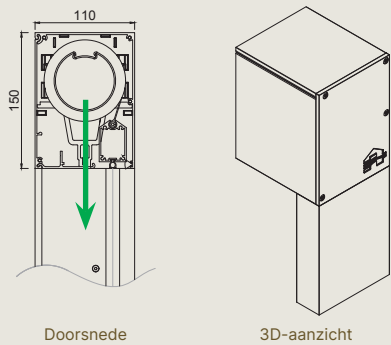
Fixscreen® 100 Slim - MS 7A - Kast
